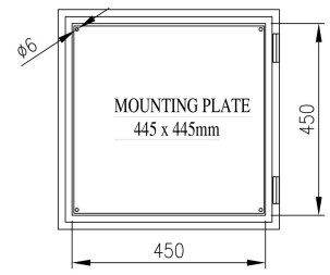
(CLEAR OPENING 450x450mm)
